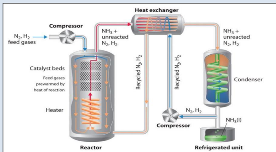
Figura 11. Reactor Haber Bosch
