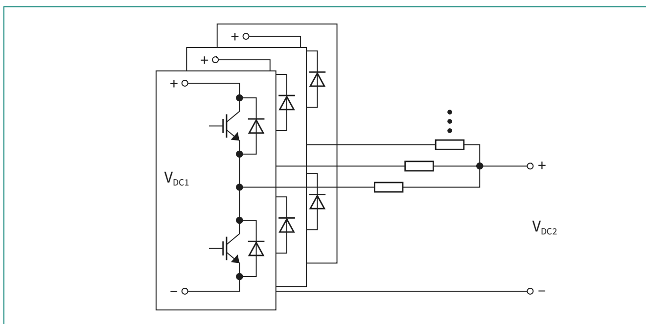
Figure 10 Interleaved buck converter [10]
