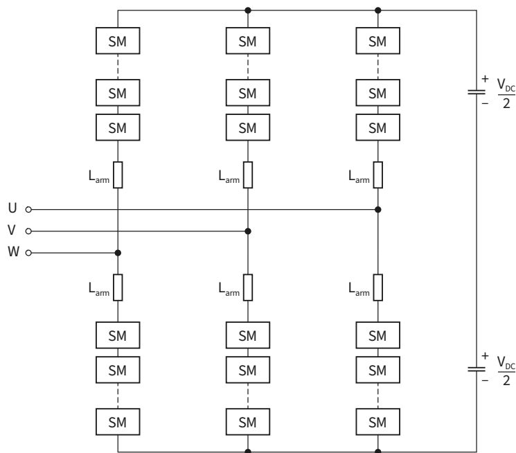
Figure 9 MMCs are now being considered for high and medium voltage DC applications, such as PCS for P2H plants [10]
