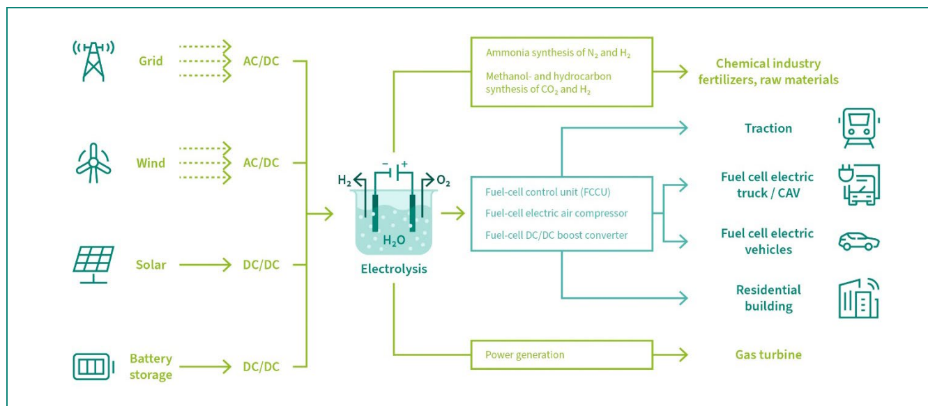
Figure 2 Hydrogen electrolysis – a part of future energy systems [4]
